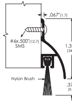
8198AA Raindrip with brush. Available D & G finishes to order at extra cost.
