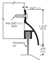
8197AA Raindrip with neoprene. Available D & G finishes to order at extra cost.
