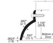
11A Raindrip. Available D & G finishes to order at extra cost.
